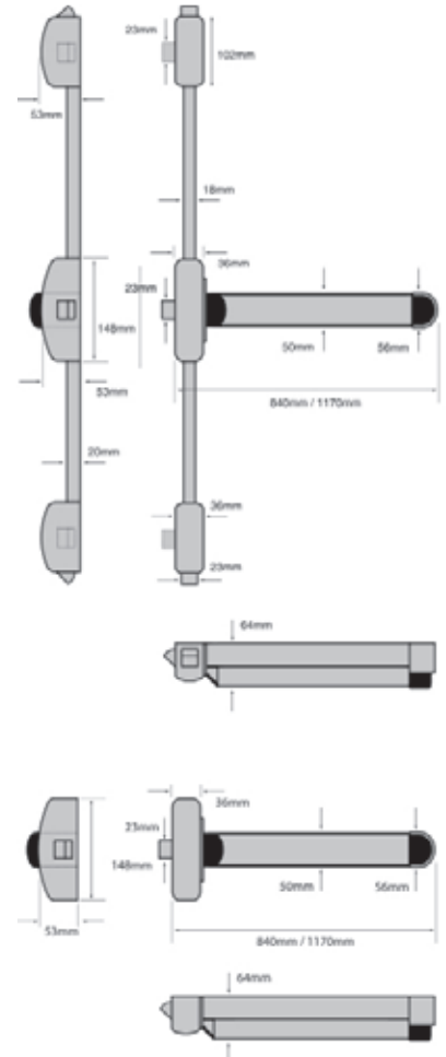
Technical drawings applicable to PHTM0, PHTM5, PHTM7
